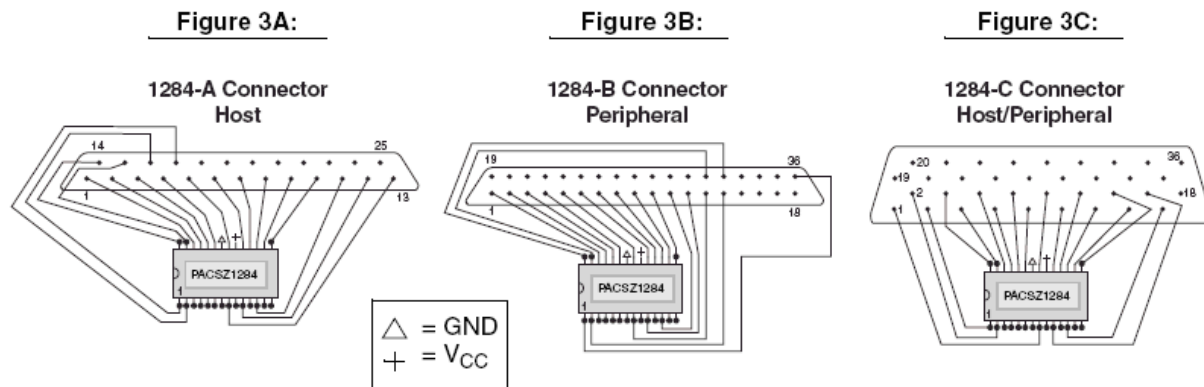
Figure 3. Example Connections of IEEE 1284 Connectors with PACSZ1284
